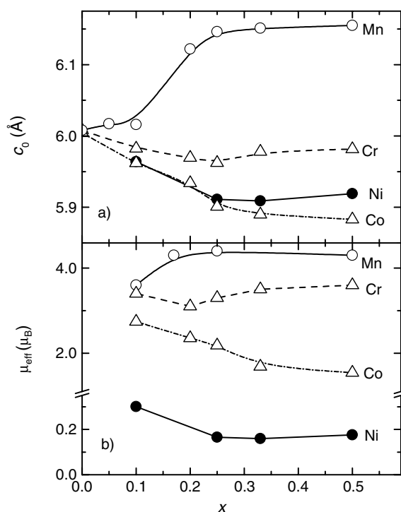
Figure 8. (a) Concentration dependences of (a) the lattice parameter c_0 and (b) the effective magnetic moment \mu_{\text{eff}} per M ion for M_x\text{TiSe}_2 systems with M = \text{Cr, Mn, Co and Ni} .
